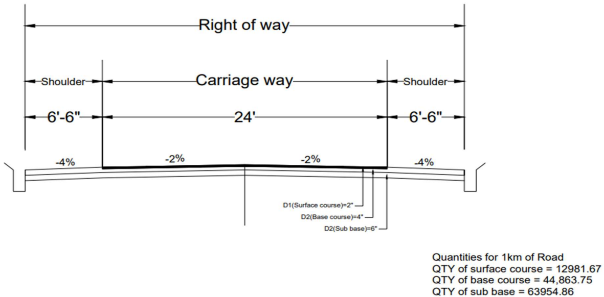
Figure-3 Typical Cross section of Nasir Bagh Road Peshawar
