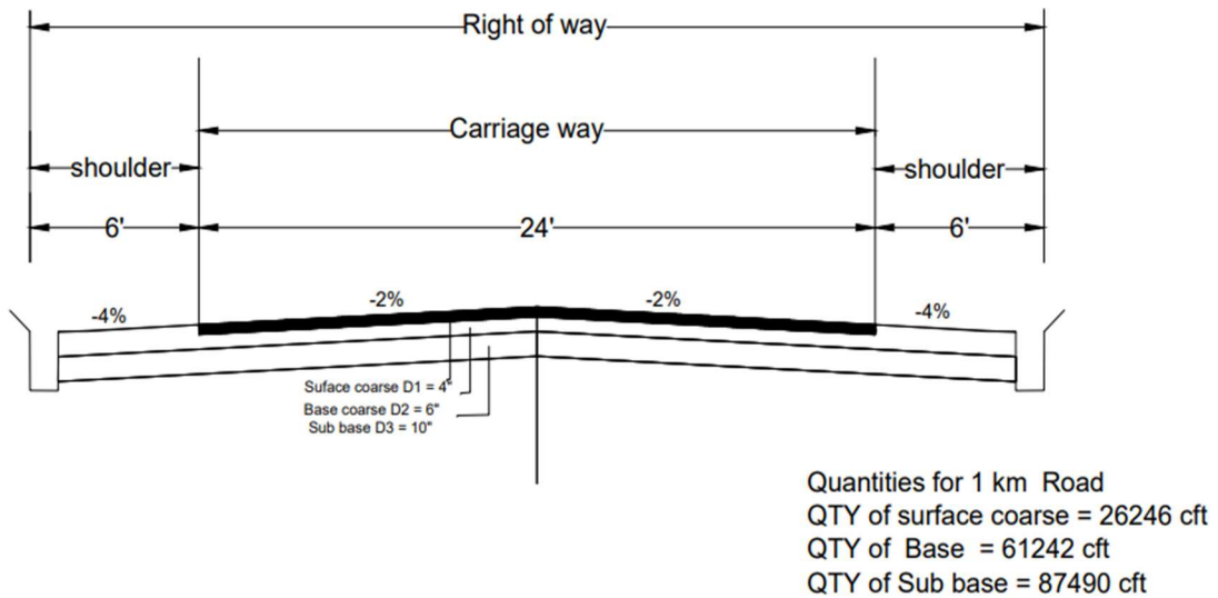
Figure-1 Typical Cross section of Topi Swabi Road Designed
