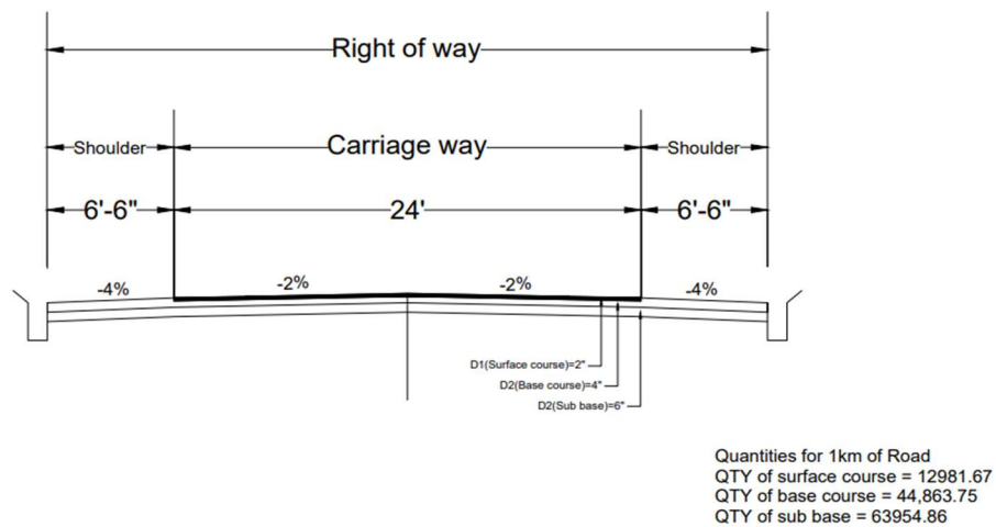
Figure-2 Typical Cross section of KDA Road Kohat
