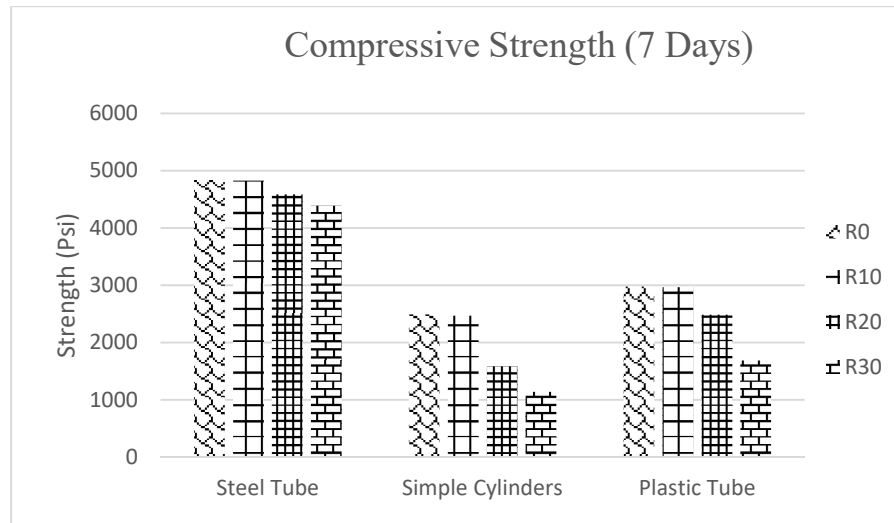
Figure-4: Compressive Test 7days
